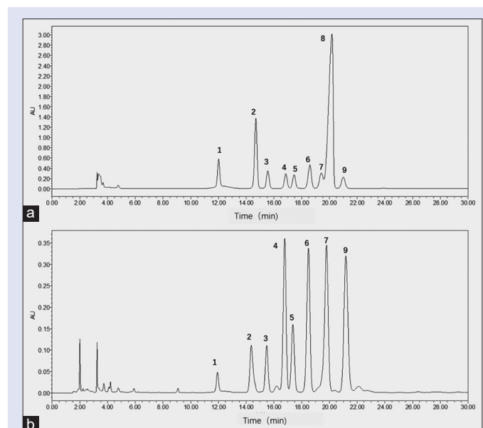
Figure 3: HPLC analysis of PMP pre-column derivatives of (a) nine standard monosaccharides. (1. mannose; 2. Ribose; 3. rhamnose; 4. galactose; 5. glucose; 6. arabinose; 7. glucuronic acid; 8. xylose; 9. galacturonic acid) and (b) CSP hydrolysate
