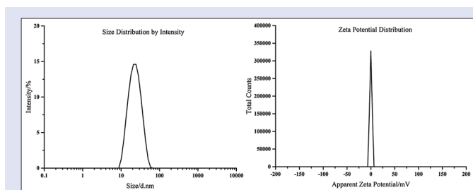
Figure 5: Particle size distribution and apparent zeta potential of Gal-SMEDDS.
