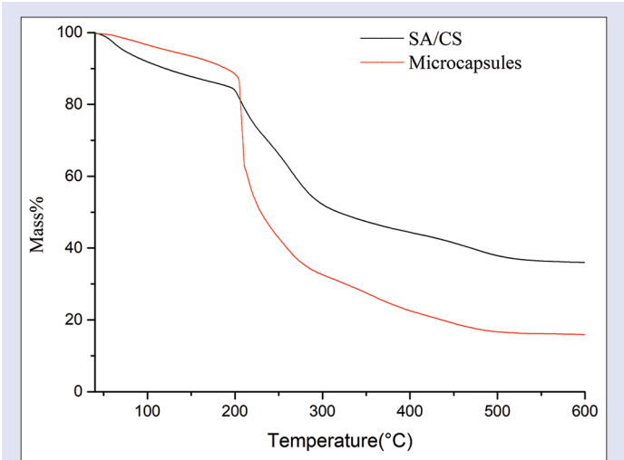
Figure 6: TG spectra of SA/CS wall and microcapsules
