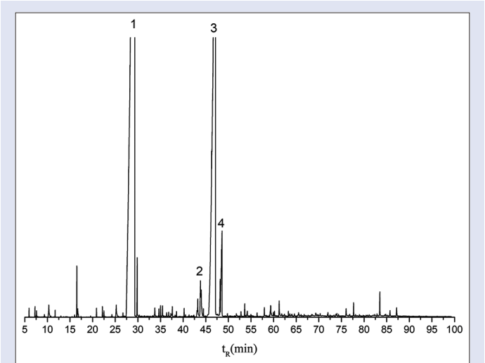
Figure 1: The GC-MS total ion flow diagram of the compound volatile oil. Peak identity: 1, cinnamaldehyde, (E)-; 2, 1 (3H)-isobenzofuranone, 3-butylidene; 3, trans-ligustilide; 4, dibutyl phthalate
