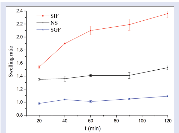
Figure 7: Swelling profiles of CVOs microcapsule at SGF (pH 1.2), NS, and SIF (pH 6.8)
