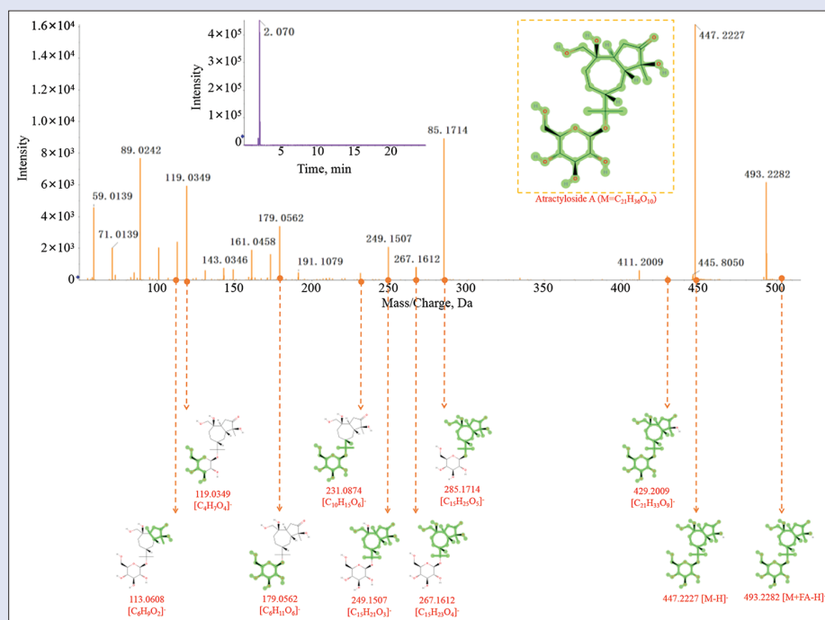
Figure 2: The MS and MS/MS information of atractylodeside A detected in Atractylodes Rhizome by UHPLC-ESI-Q-TOF-MS/MS
