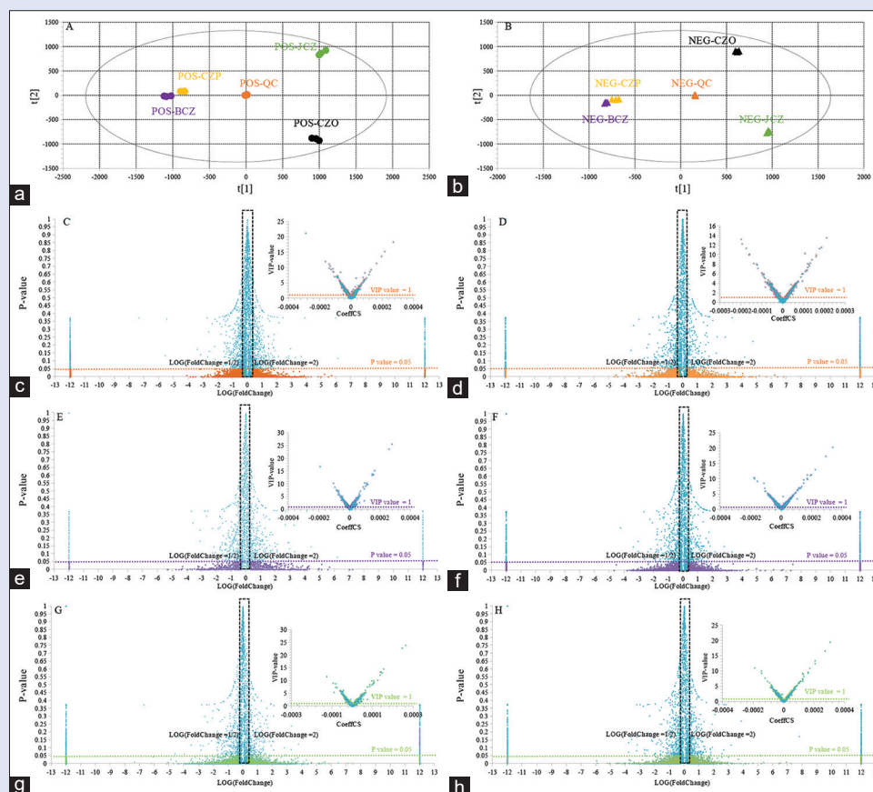
Figure 3: The principal component analysis (PCA) and Variable importance in the projection (VIP) analysis of different processed products of Atractylodes Rhizome in positive ion mode and negative ion mode (a) PCA analysis in positive ion mode (b) PCA analysis in negative ion mode (c) VIP analysis (cangzhu pieces – CZP vs. cangzhu – CZO) in positive ion mode (d) VIP analysis (CZP vs. CZO) in negative ion mode (e) VIP analysis (bran frying cangzhu – BCZ vs. cangzhu CZO) in positive ion mode (f) VIP analysis (BCZ vs. CZO) in negative ion mode (g) VIP analysis (Jiao cangzhu – JCZ vs. cangzhu – CZO) in positive ion mode (h) VIP analysis (JCZ vs. CZO) in negative ion mode
