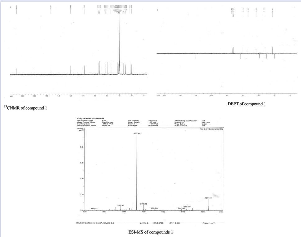
Figure 1: 13CNMR spectrum and MS spectrum of compound 1
