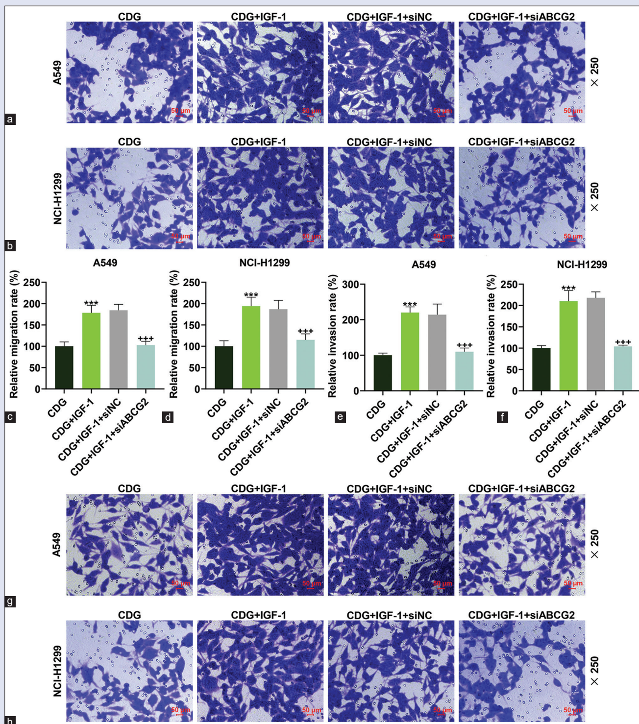
Figure 6: Combination of Vinorelbine with oxaliplatin repressed NSCLC cell migration and invasion via PI3K/AKT/ABCG2 axis. (a) Representative images of A549 cell migration through Transwell assay after treatment of vinorelbine, oxaliplatin, and IGF-1 and transfection of siABCG2 (scale: 50 \mu m; magnification: \times 250 ). (b) Representative images of NCI-H1299 cell migration through Transwell assay after treatment of vinorelbine, oxaliplatin, and IGF-1 and transfection of siABCG2 (scale: 50 \mu m; magnification: \times 250 ). (c) The migration rate of A549 cells was tested by Transwell assay after treatment of vinorelbine, oxaliplatin, and IGF-1 and transfection of siABCG2. (d) The migration rate of NCI-H1299 cells was tested by Transwell assay after treatment of vinorelbine, oxaliplatin, and IGF-1 and transfection of siABCG2. (e) The invasion rate of A549 cells was tested by Transwell assay after treatment of vinorelbine, oxaliplatin, and IGF-1 and transfection of siABCG2. (f) The invasion rate of NCI-H1299 cells was detected by Transwell assay after treatment of vinorelbine, oxaliplatin, and IGF-1 and transfection of siABCG2. (g) Representative images of A549 cell invasion through Transwell assay after treatment of vinorelbine, oxaliplatin, and IGF-1 and transfection of siABCG2 (scale: 50 \mu m; magnification: \times 250 ). (h) Representative images of NCI-H1299 cell invasion through Transwell assay after treatment of vinorelbine, oxaliplatin, and IGF-1 and transfection of siABCG2 (scale: 50 \mu m; magnification: \times 250 ). *** P < 0.001 vs. CDG group; +++ P < 0.001 vs. CDG+IGF-1 + siNC group. All experiments were repeated independently at least three times. Data were shown as the means \pm standard deviation. NSCLC, non-small cell lung cancer; siABCG2, silencing ABCG2; CDG, the group co-treated with vinorelbine and oxaliplatin; siNC, the negative control for siABCG2.
