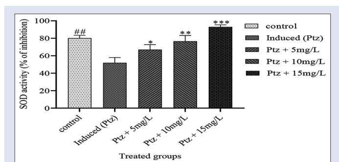
Figure 10: SOD assay
