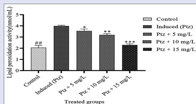
Figure 9: LPO assay
