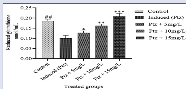
Figure 8: GSH activity
