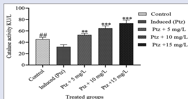
Figure 7: Catalase activity
