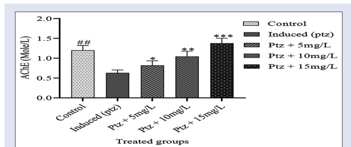
Figure 11: AChE assay
