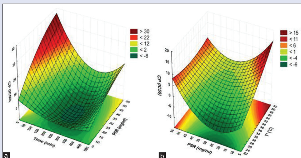
Figure 7: (a) Three-dimensional response surface plots showing the effect of time (min) and plant-to-solvent ratio (PSR) on the chelating power activity for E. officinarum ; Effect of temperature T^\circ (°C) and PSR on the chelating power activity for (b) E. officinarum
