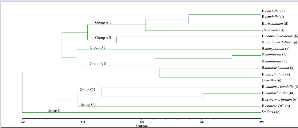
Figure 1: UPGMA phenogram of Bupleurum genera clustered given morphological characteristics
