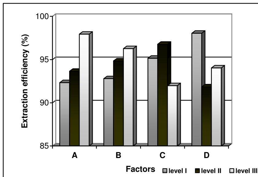
Fig. 2 Extraction efficiency (%) obtained under orthogonal design conditions.
