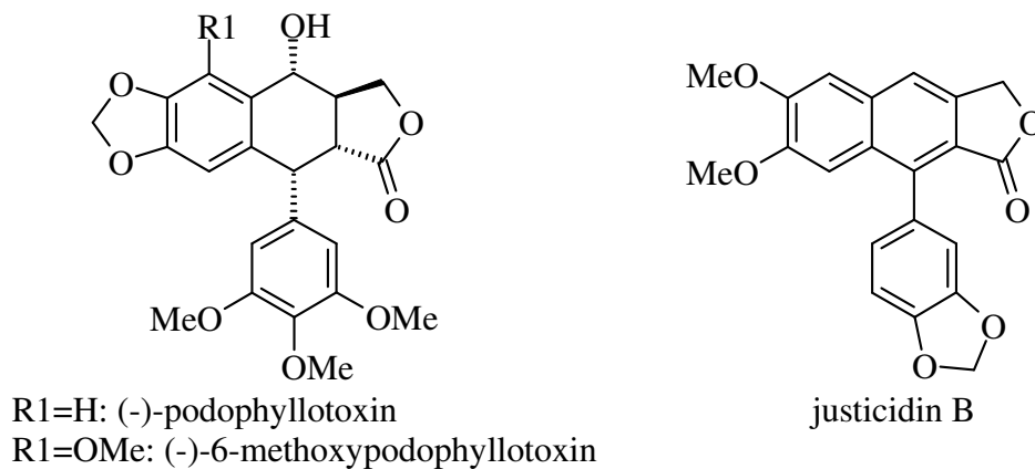
Fig. 1: Chemical structures of some of identified lignans
