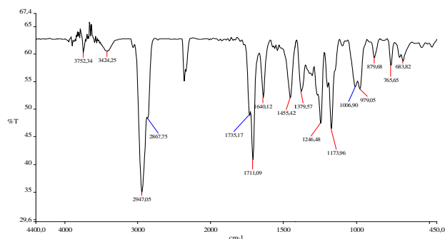
Figure 2. JANA-1 infrared spectra
