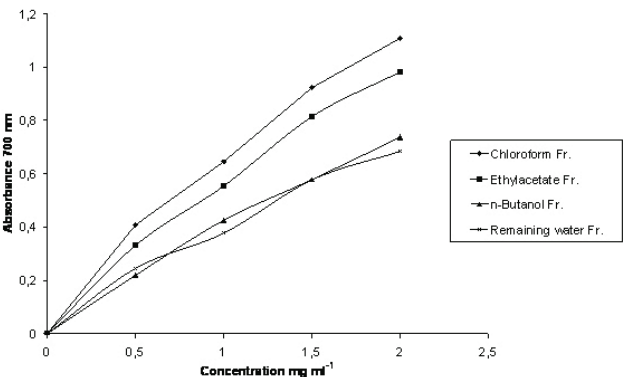
Figure 1: Reducing power of R. canina fractions (0.5, 1, 1.5 and 2 mg ml -1 ). BHA (Abs700 nm; 1.749, 3.569 and 3.677 for 50, 250 and 500 µg ml -1 , respectively) was used as reference antioxidant for comparison.
