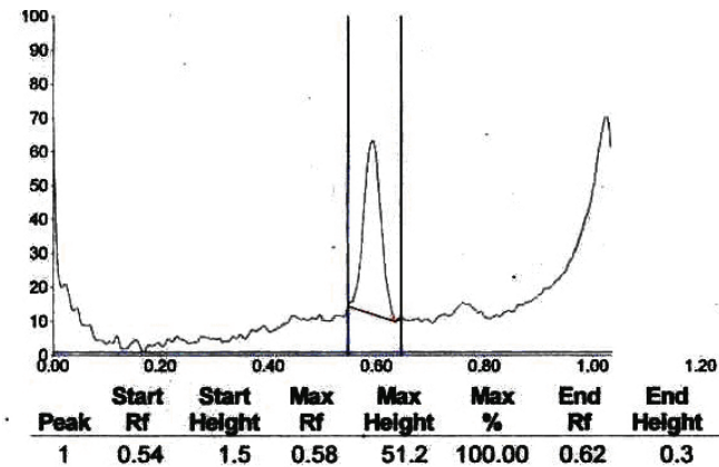
Figure 3: HPTLC chromatogram of R. dumetorum (sample)
