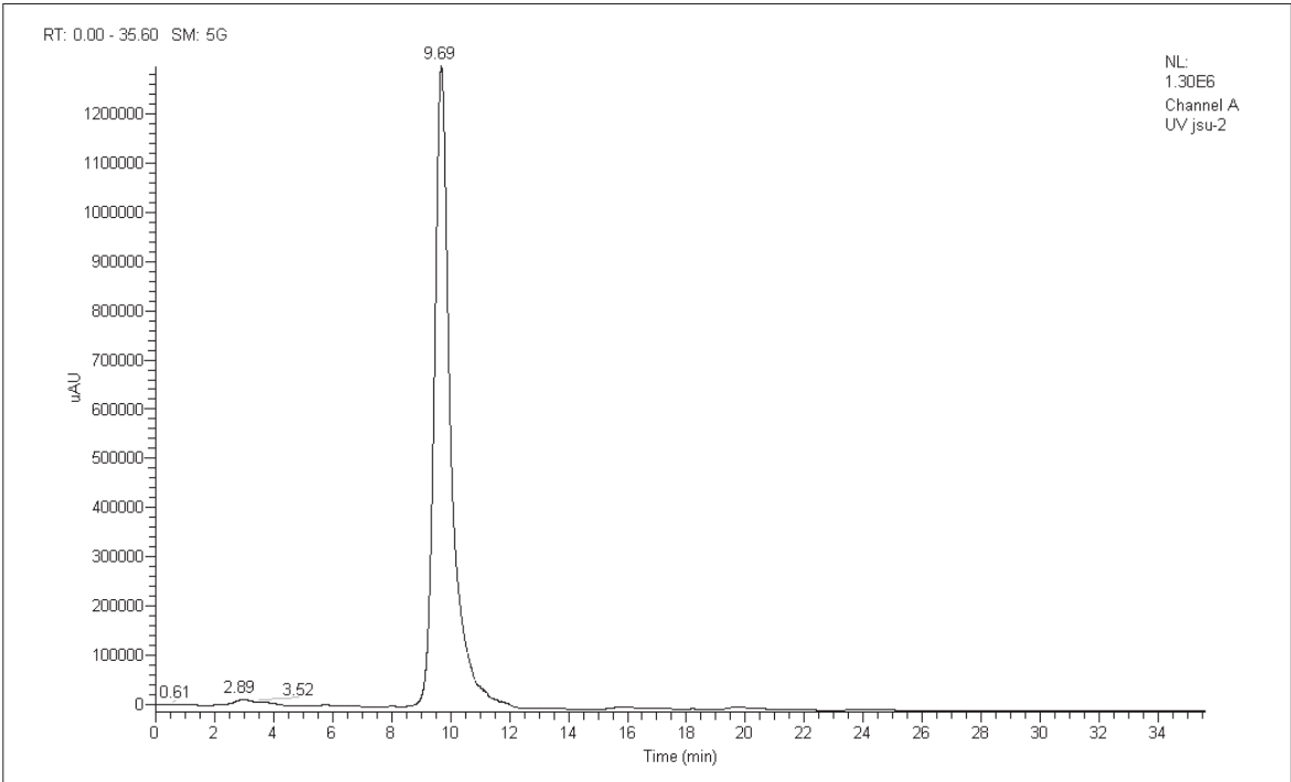
Figure 2: UV chromatogram of the molluscicidal ingredient
