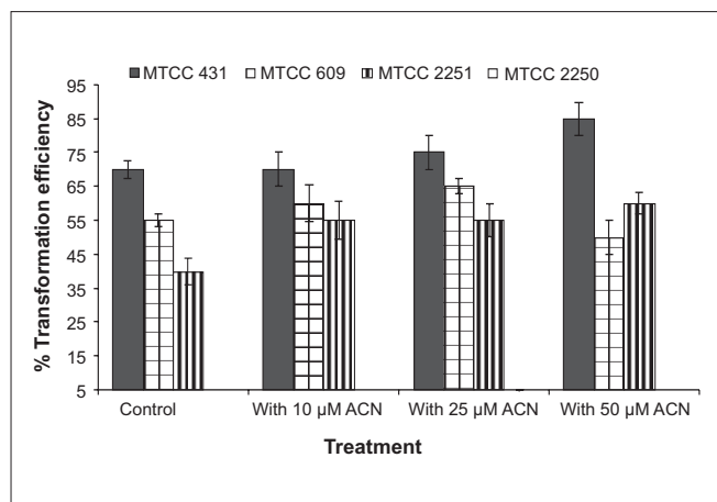
Figure 1: Effect of acetosyringone on the (%) transformation efficiency of A. precatorius * leaf explants. (*30 explants were used in each treatment. No transformation was found with MTCC 2250 strain with any treatment. Average values are given; error bars are represented as vertical lines)
